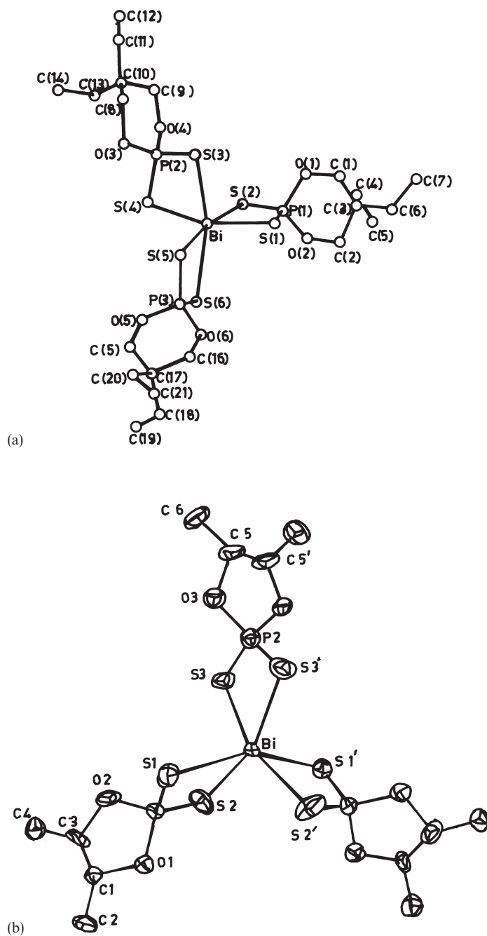
Fig. 2. Ortep plot of (a) \text{Bi} \left[ \text{S}_2\text{P} \begin{array}{c} \text{O}-\text{CH}_2 \\ \text{O}-\text{CH}_2 \end{array} \text{CEt}_2 \right]_3 and (b) \text{Bi} \left[ \text{S}_2\text{P} \begin{array}{c} \text{OCHCH}_3 \\ \text{OCHCH}_3 \end{array} \right]_3 . [R. Bohra, H.P.S. Chauhan, G. Srivastava and R.C. Mehrotra, Phosphorus, Sulfur and Silicon , 60 (1991) 167. Reproduced with permission].
