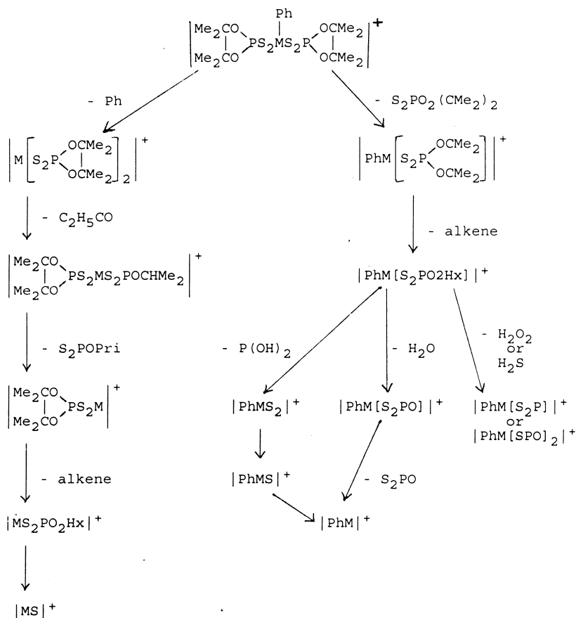
Scheme 1. R.K. Gupta, A.K. Rai, R.C. Mehrotra and V.K. Jain, Inorg. Chim. Acta , 88 (1984) 201–207. Reproduced with permission.
